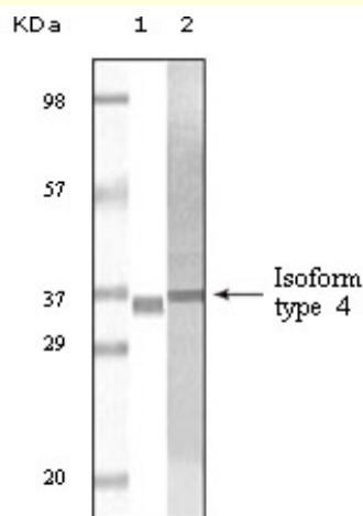
Figure 1: Western blot analysis using anti-Human MAPK10(isoform type 4) monoclonal antibody against recombinant MAPK10(lane 1) and NIH3T3 cell
